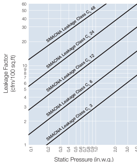
Figure 1 Based on SMACNA (HVAC Air Duct Leakage Test Manual First Edition 1985) Figure 4-1 'Duct Leakage Classification'
